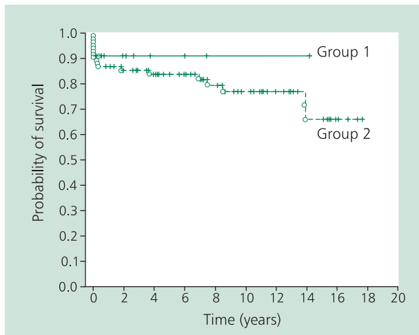
Figure 4. Kaplan-Meier survival curves
